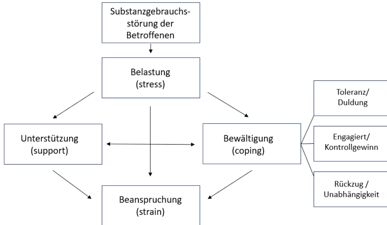
Stress-Strain-Coping-Support-Modell
